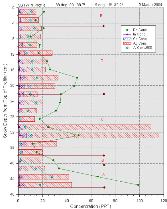
Figure 4. Concentrations of trace chemical elements versus depth in the TWIN snow profile of 5 March 2004. Storm periods A - E from Fig. 3 are shown between dark red horizontal lines.
